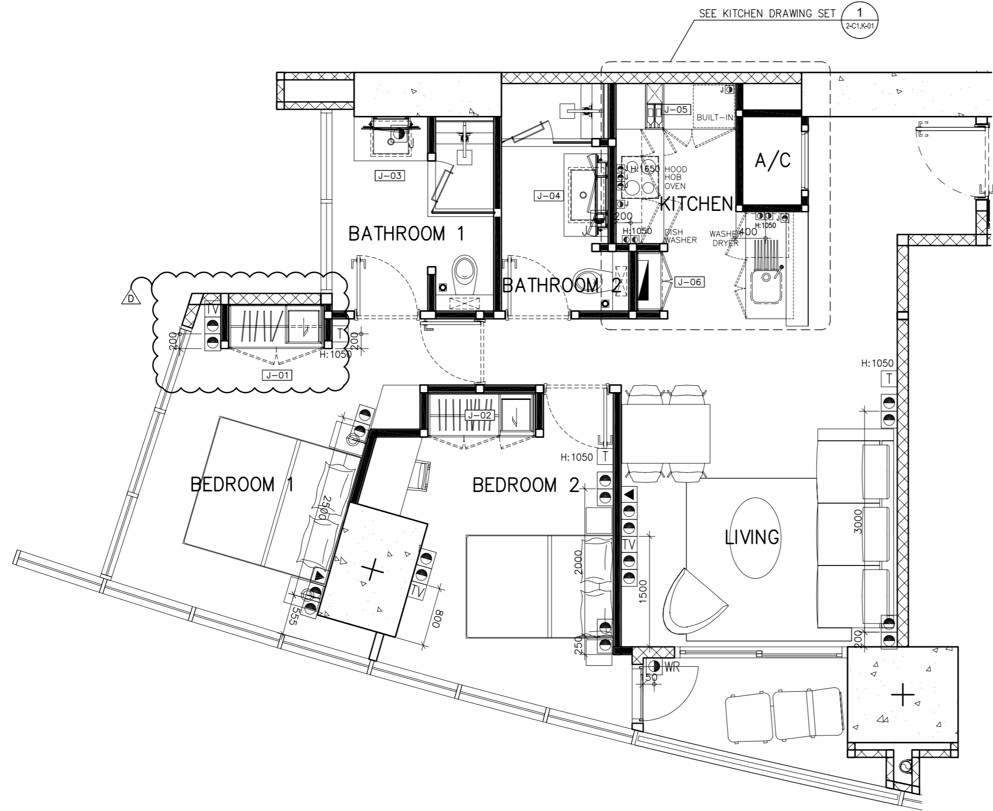
A FURNITURE & ELECTRICAL PLAN SCALE: 1:50
